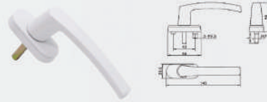
SLIDING HANDLE
